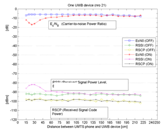
Fig. 21. Measured parameters of the UMTS terminal connected to the real network.
