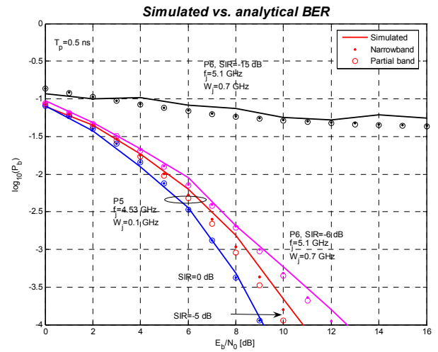
Figure 5. BER using different waveforms with different SIR.
