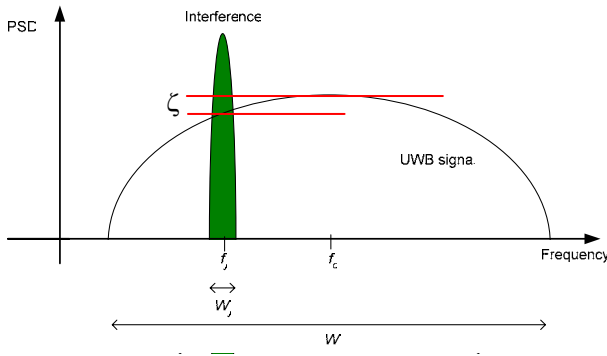
Figure 1. Power spectral densities presented for the desired UWB and interfering signals.
