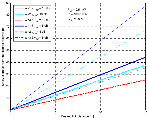
Figure 6. Minimum interference distance between WLAN and UWB; WLAN is interfering UWB.
