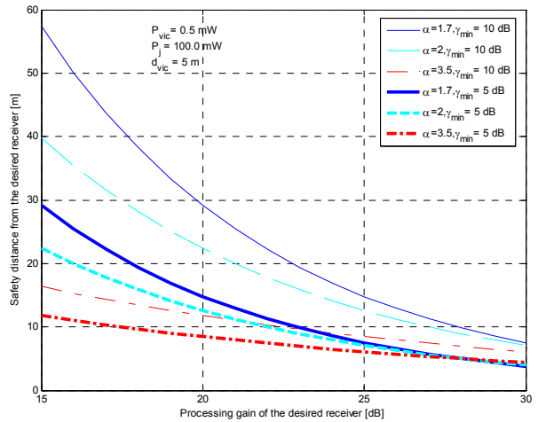
Figure 8. WLAN impact on UWB as a function of UWB processing gain. Desired link distance is 5 m.
