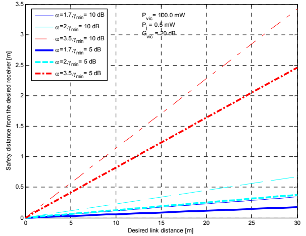
Figure 7. Minimum interference distance between WLAN and UWB; UWB is interfering WLAN.
