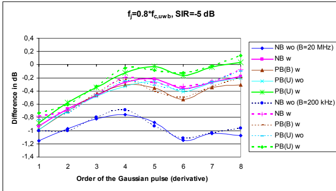
Figure 8. Difference between analytical and simulated results; f_j = 0.8f_c, W_j = 200 MHz and 20 MHz, SIR = -5 dB.
