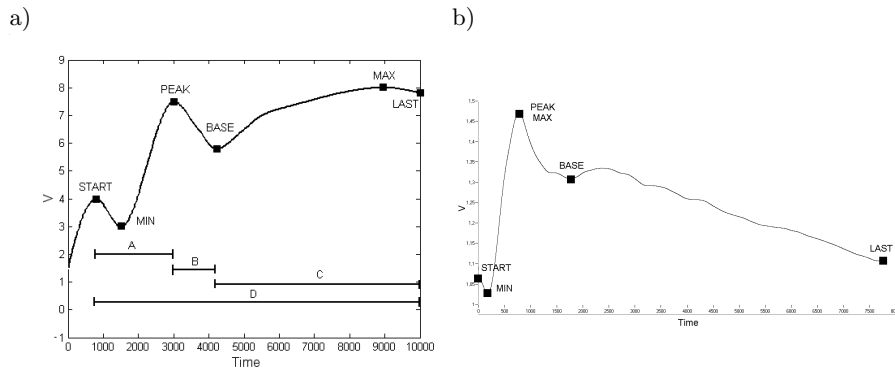
Fig. 2. a) The geometrical features on an artificial voltage curve. The line segments A-D below the curve demonstrate the intervals based on the transition points on which means were calculated. b) An example of how the geometrical features often partially overlap in practice. On this voltage curve, the features 'peak' and 'max' overlap
